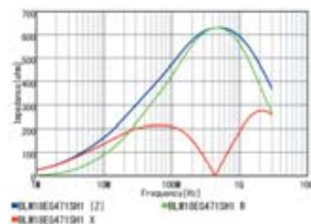
BLM18EG471SZ1/BLM18EG471SH1
