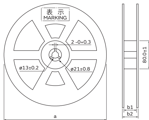
REEL DETAILS (HEAW/HEAWS)
