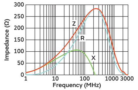
BLL18AG221A2E1H01/BLL18AG221DBE1H01
