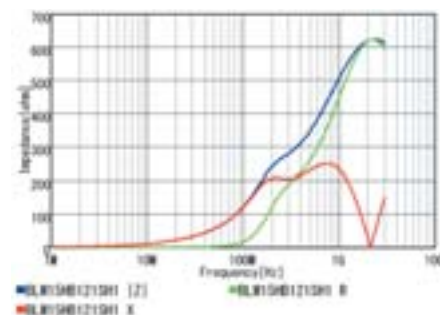
BLM15HB121SZ1/BLM15HB121SH1
