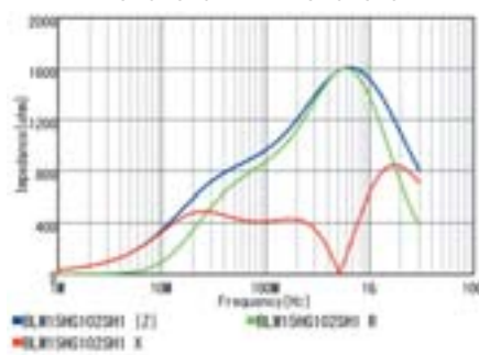
BLM15HG102SZ1/BLM15HG102SH1
