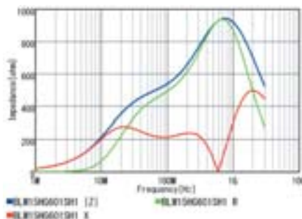
BLM15HG601SZ1/BLM15HG601SH1
