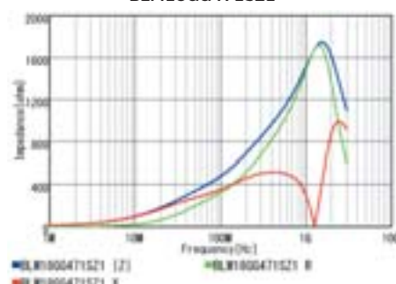
BLM18GG471SZ1
