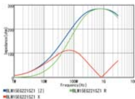
BLM15EG221SZ1/BLM15EG221SH1
