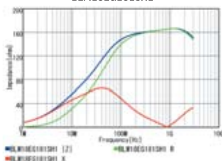
BLM18EG181SH1
