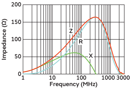
BLL18AG121A2E1H01/BLL18AG121DBE1H01
