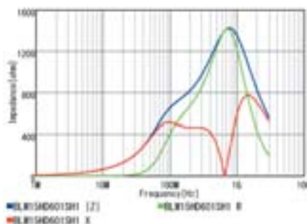
BLM15HD601SZ1/BLM15HD601SH1
