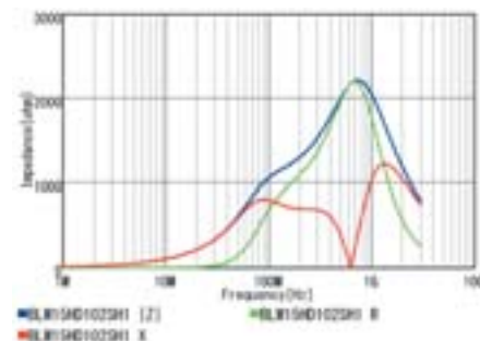
BLM15HD102SZ1/BLM15HD102SH1
