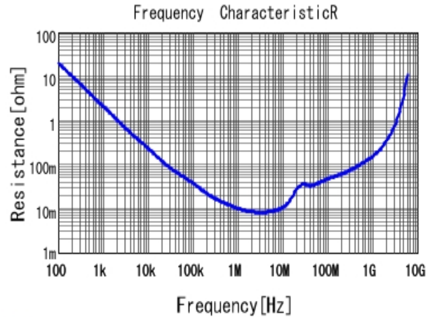
■ GRM188R11C474KA88 R DC0V, 20degC
