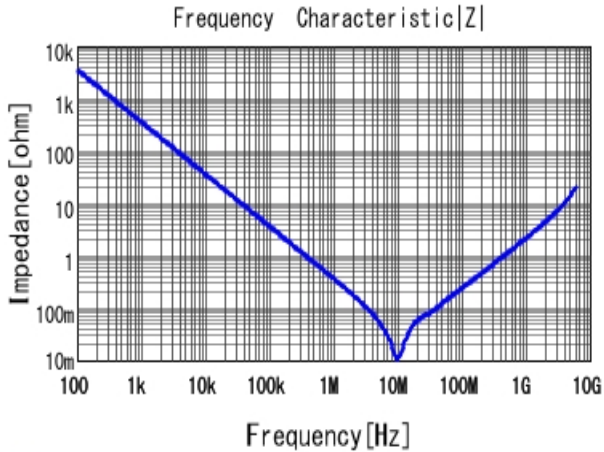
■ GRM188R11C474KA88 |Z| DC0V, 20degC
