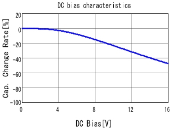
■ GRM188R11C474KA88 C-DC bias capchange, 20.0degC, AC1.
