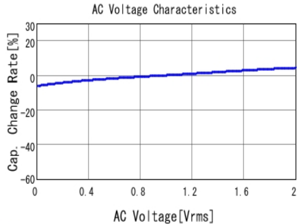
■ GRM188R11C474KA88 C-AC Voltage capchange, DC0V, 20.0d
