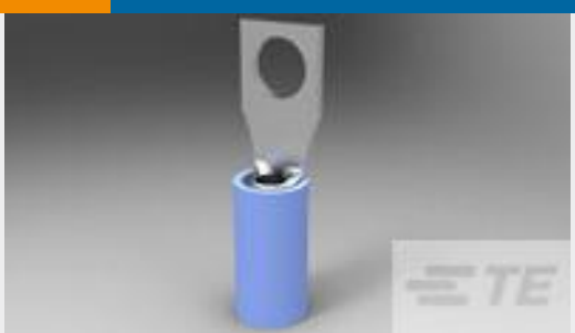
TE Part #2-327946-4 TERMINAL,PIDG RECT 16-14 8
