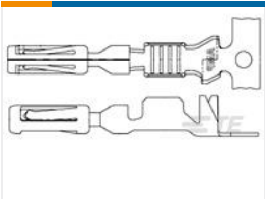
TE Part #770520-1 AMPSEAL, TERMINAL, TIN PLATE, 16-20AWG WIRE
