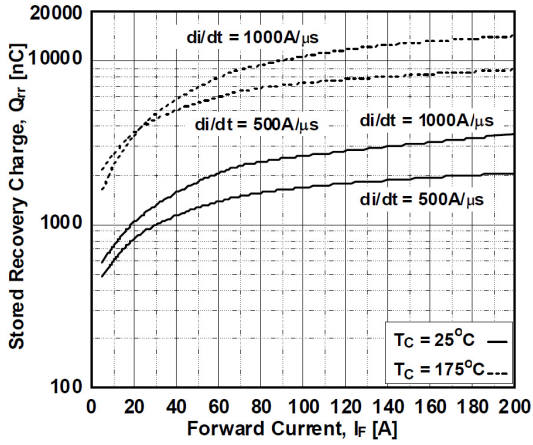
Figure 21. Stored Charge
