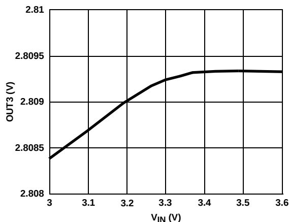
FIGURE 9. OUT3 LINE REGULATION
