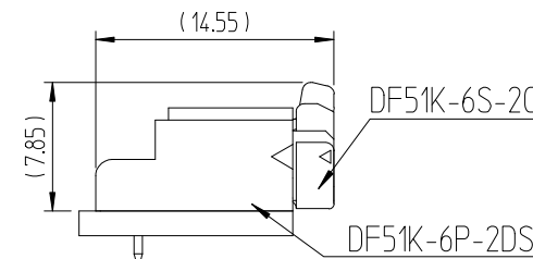
ENGAGEMENT FIGURE (2:1)
