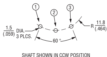
SHAFT SHOWN IN CCW POSITION
