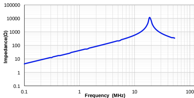
VSAB0630-6R8M
