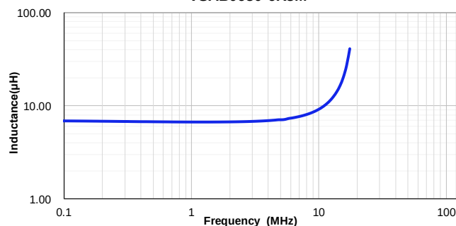
VSAB0630-6R8M
