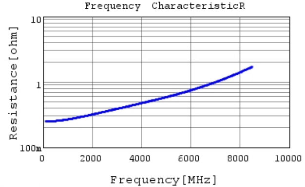
GRM0335C2A3R2WA01 R DCOV, 25degC
