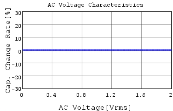
GRM0335C2A3R2WA01 C-AC Voltage capchange, Dc
