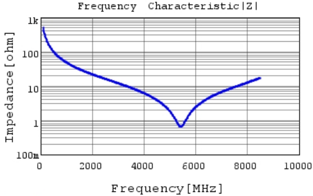
GRM0335C2A3R2WA01 |Z| DCOV, 25degC
