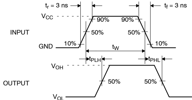
Figure 6. AC Waveforms
