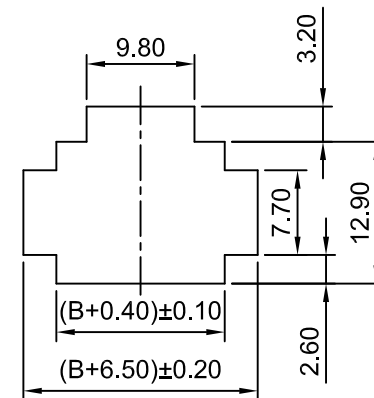
Panel Hole Layout Thickness:0.90~1.30
