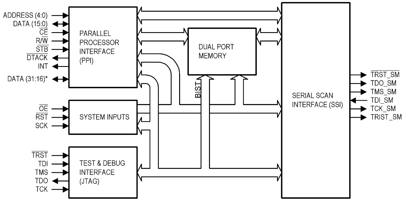
Figure 1. SCANSTA101 STA Master and Interfaces
