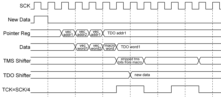
Figure 8. Timing from Mode Register Write to Vector Start
