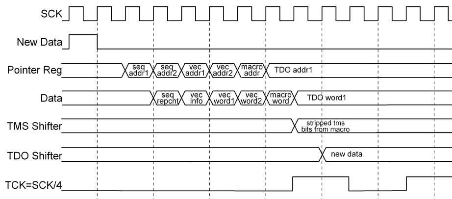
Figure 9. Timing from Mode Register to Sequencer Start
