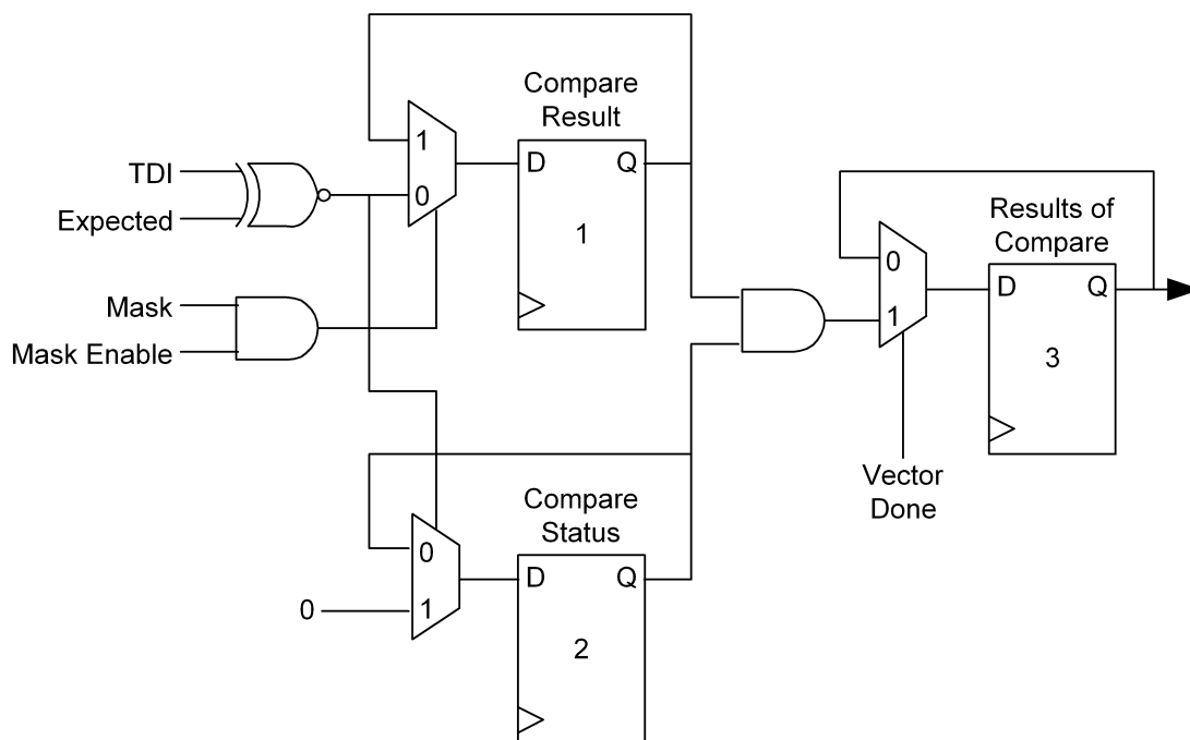
Figure 7. Compare Logic
