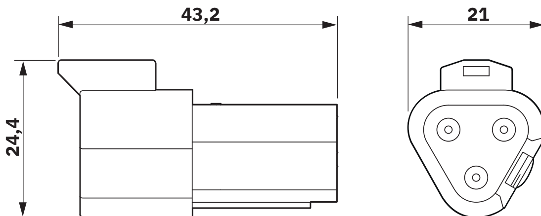
AT04-3P top view and side view
