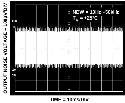
Figure 13. Broadband Noise
