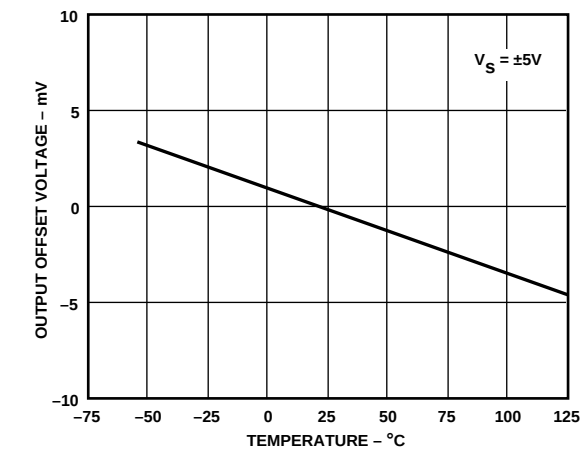
Figure 37. Output Offset Voltage ( Z_{OS} ) vs. Temperature
