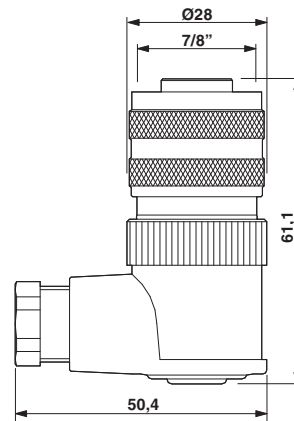
Dimensioned drawing
