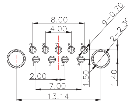
REFERENCE PCB LAYOUT
