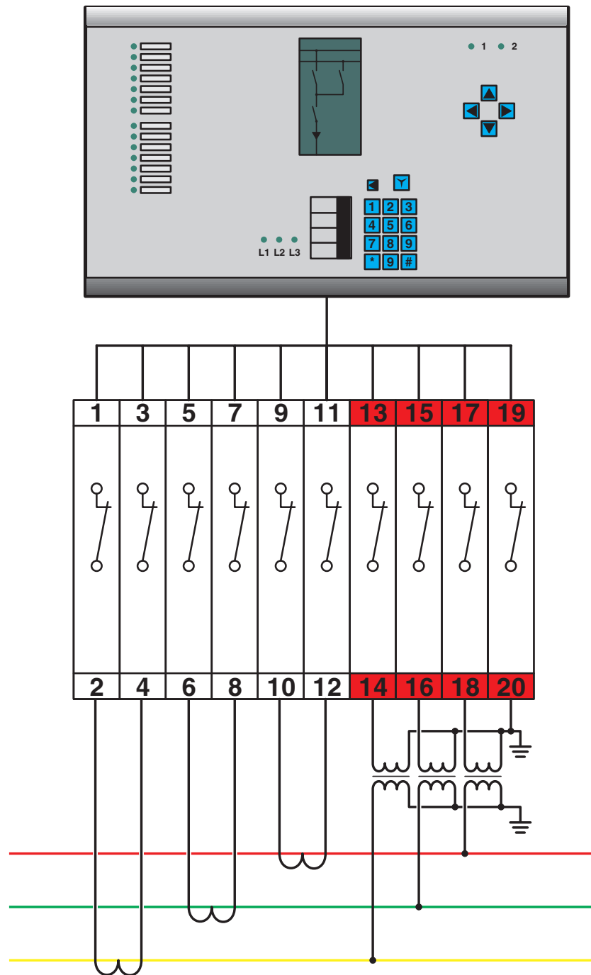
Circuit diagram
