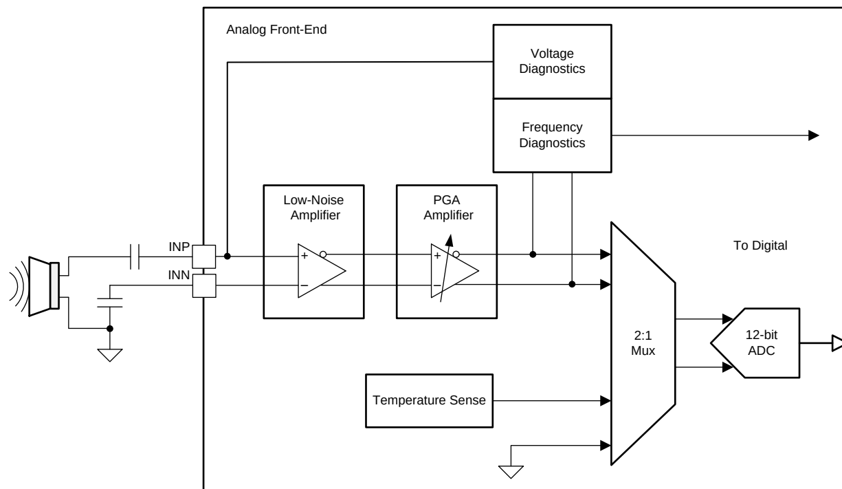
Figure 5. Analog Front-End
