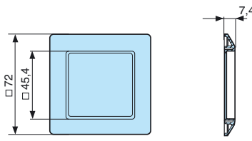
26546842 - Adaptor for 72 x 72 mm cut-out
