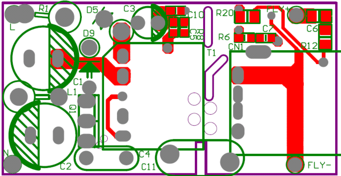
Figure 36. Front Side
