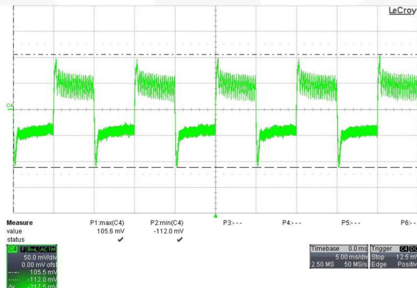
Figure 12. 115V / 60Hz at Step Response
