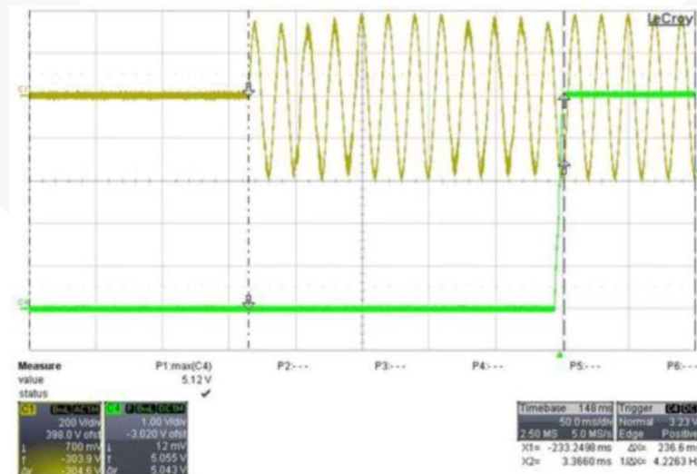
Figure 4. 264V / 50Hz at Maximum Load
