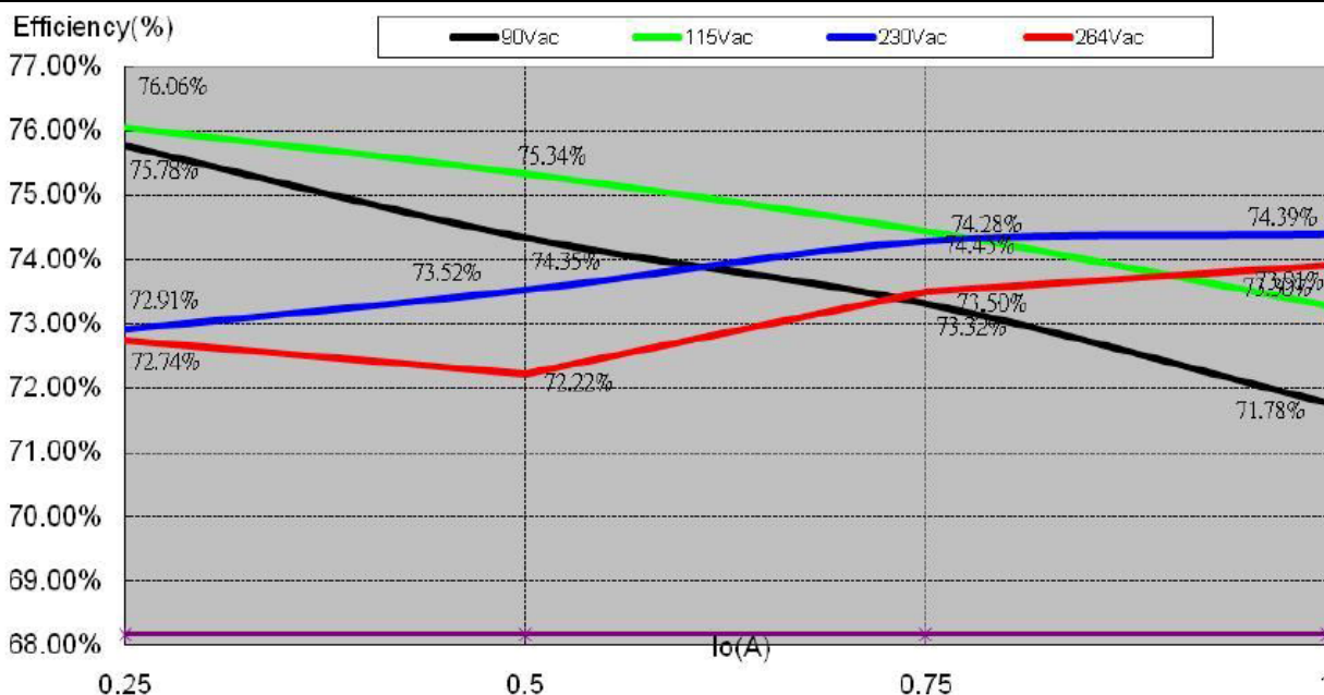
Figure 9. Efficiency Chart
