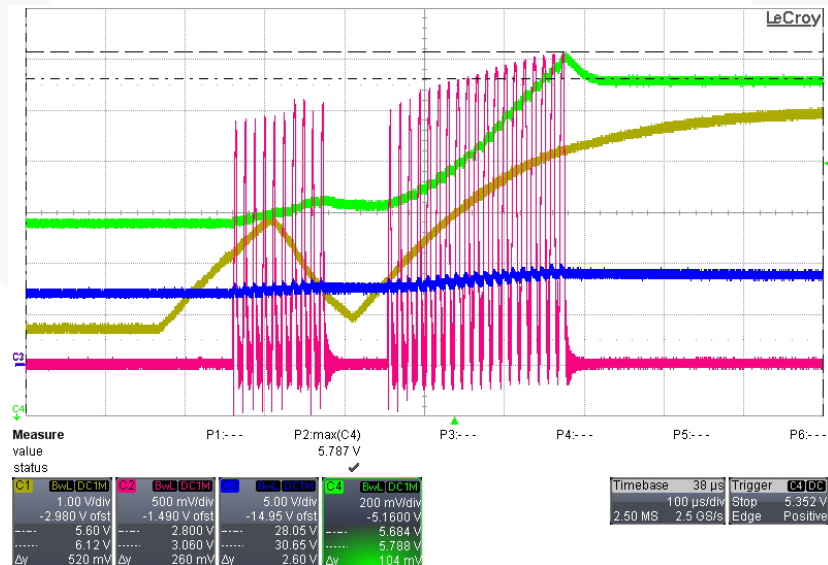
Figure 29. 264V AC Minimum Load
