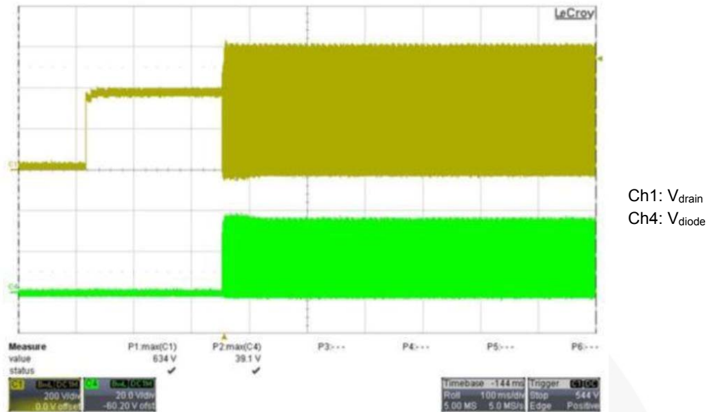
Figure 25. 264V / 50Hz at Maximum Load Startup
