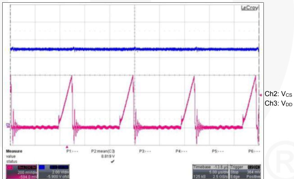
Figure 19. 90V / 60Hz at Maximum Load
