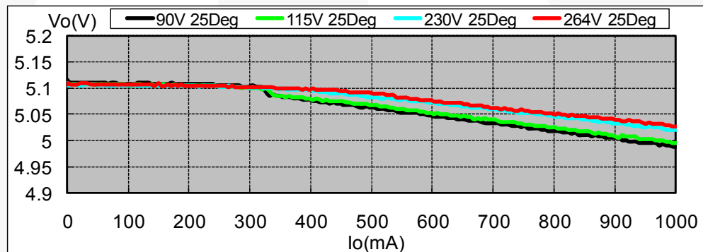
Figure 26. Constant Voltage Curve
