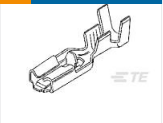
TE Part #63442-1 PL 250 TERMINAL REC 18-14 AWG TPBR
