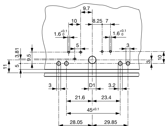
Drilling Diagram / CMF3 (C6)
