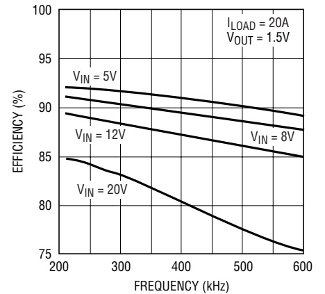
Efficiency vs Frequency (Figure 14)
