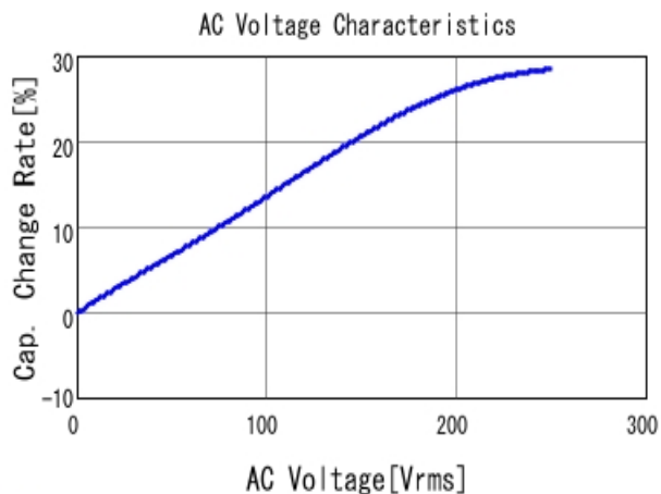
■ DE1E3RA472MA4BN01F C-AC Voltage capchange, DCOV, 20.0
