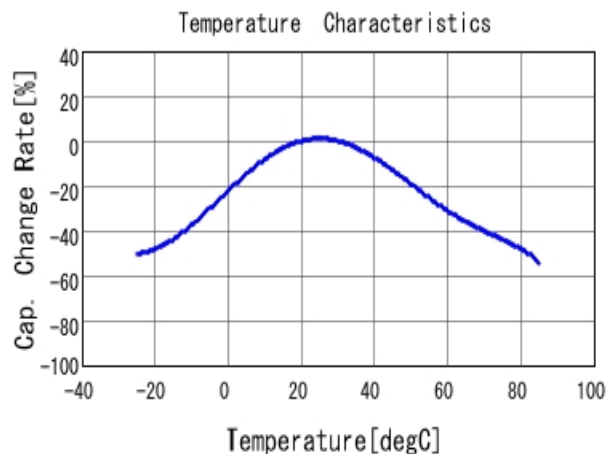
■ DE1E3RA472MA4BN01F C-Temp. capchange, DCOV, AC1Vrms
