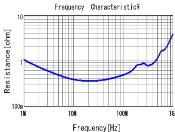
■ DE1E3RA472MA4BN01F R DCOV, 20degC
