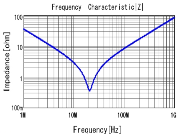
■ DE1E3RA472MA4BN01F |Z| DCOV, 20degC
