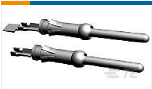
TE Part #1-66359-1 III+ PIN, 18-14, TIN-LEAD, STRIP
