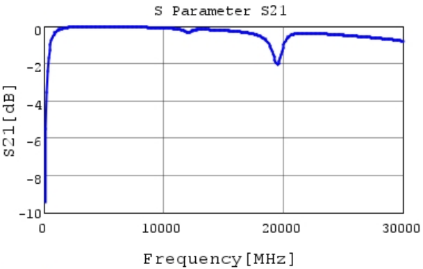
GJM0335C1E5R7CB01 S21 DCOV, 25degC
