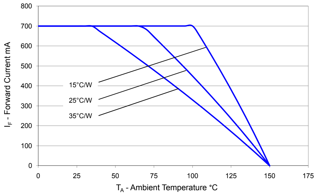
Figure 18. Maximum forward current vs. ambient temperature, based on T_{J\text{MAX}} = 150^{\circ}\text{C} .
