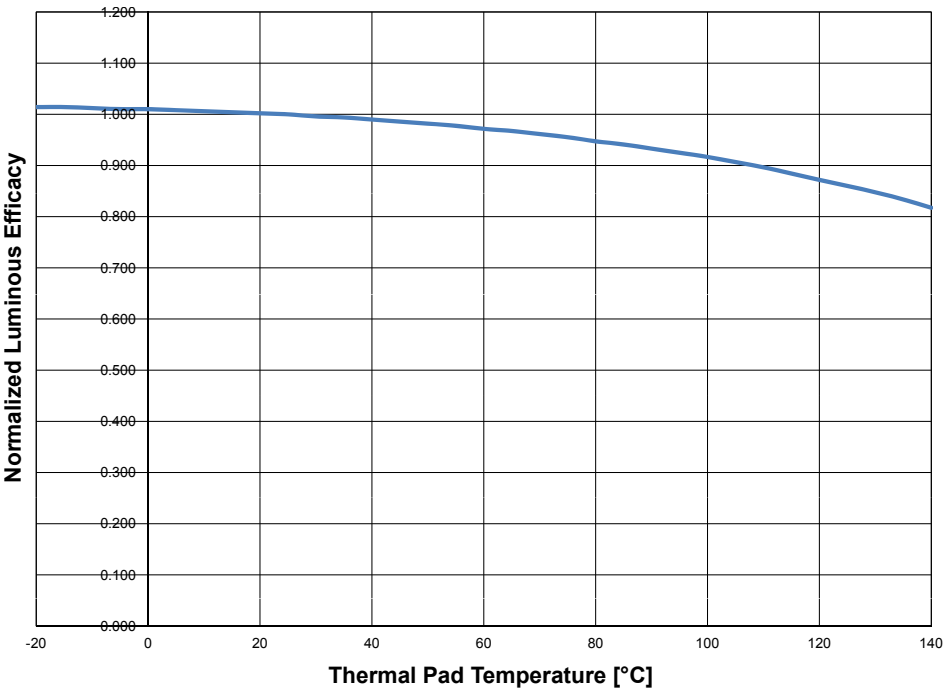
Figure I6. Relative luminous efficacy vs. thermal pad temperature, test current 700 mA.
