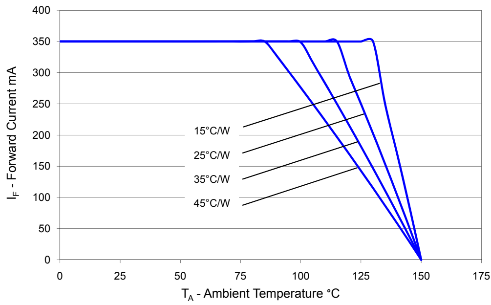
Figure 17. Maximum forward current vs. ambient temperature, based on T_{J\text{MAX}} = 150^{\circ}\text{C} .
