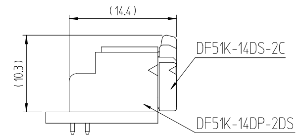
ENGAGEMENT FIGURE (2:1)
