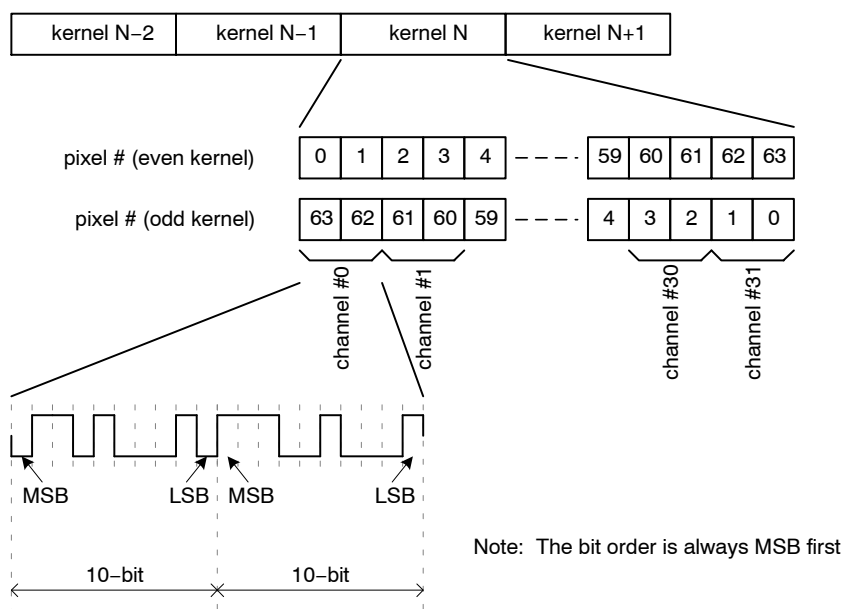
Figure 36. 32 LVDS Data Output Order when Subsampling is Disabled
