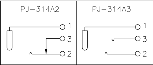
CIRCUIT DIAGRAM
