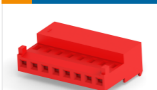
TE Part #3-644042-6 Nylon Gold Plated Receptacle: 2.54 mm, with Mating Alignment, MTA 100
