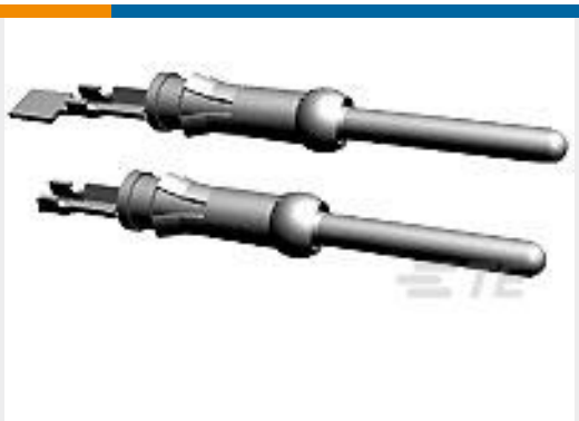
TE Part #66597-2 III+ PIN,18-14,30AU/FL,STRIP
