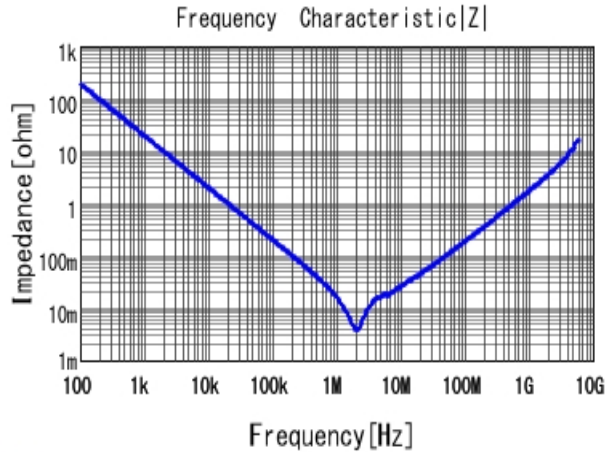
■ GRM21BB31A106KE18 |Z| DC0V, 20degC
