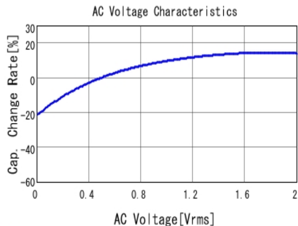
■ GRM21BB31A106KE18 C-AC Voltage capchange, DC0V, 20.0d
