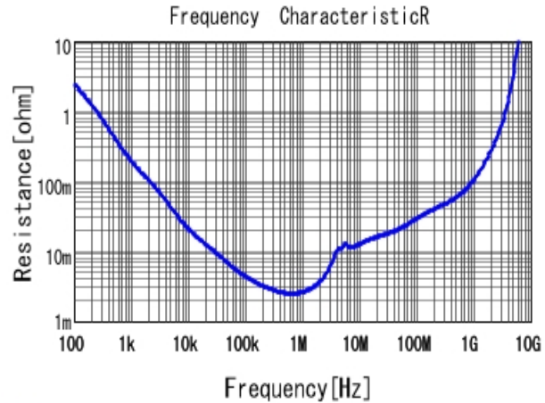
■ GRM21BB31A106KE18 R DC0V, 20degC
