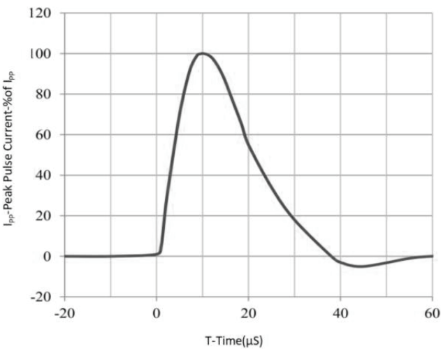
EC61000-4-5 Waveform( 8/20μs pulse)
