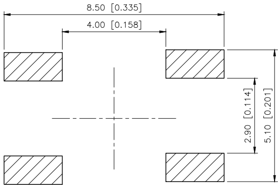
SMD REFLOW PATTERN(N/S:±0.1)
