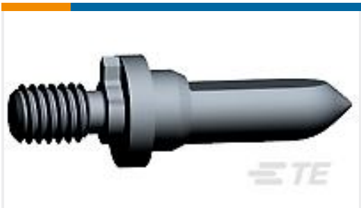
TE Part #2000676-3 Keyed Guide Pin, Machined, Vita 46
