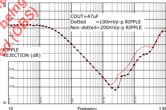
Fig. 13: PSRR, 50mA, 1.5VIN, 1VOUT, 47μF COUT
