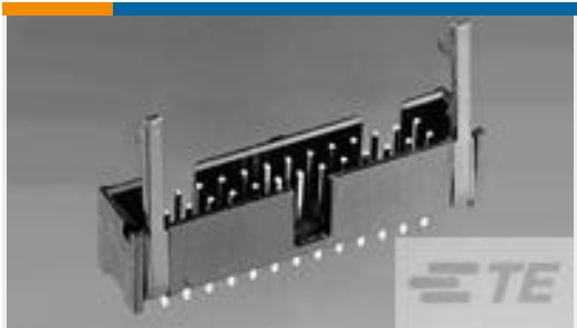
TE Part # 3-1761712-5 IDC LOW PRO HDR 50P RA LG LAT
