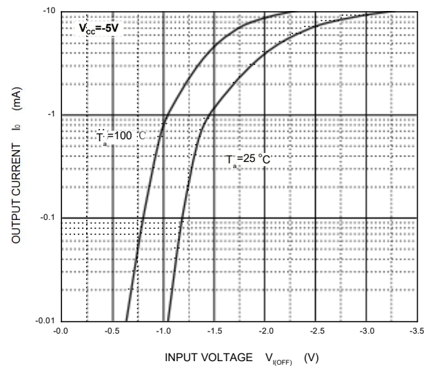
OFF Characteristics
