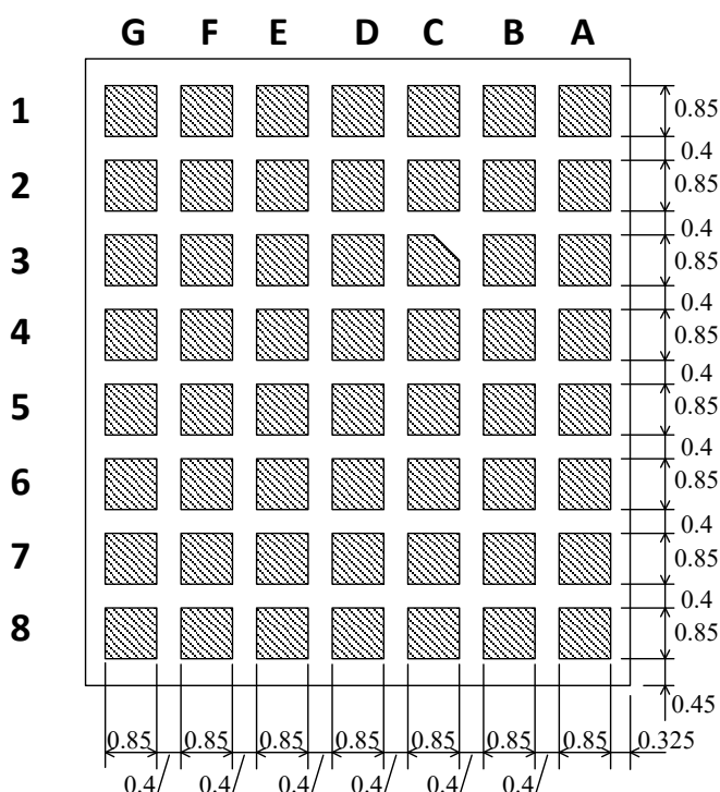
< Bottom View >
