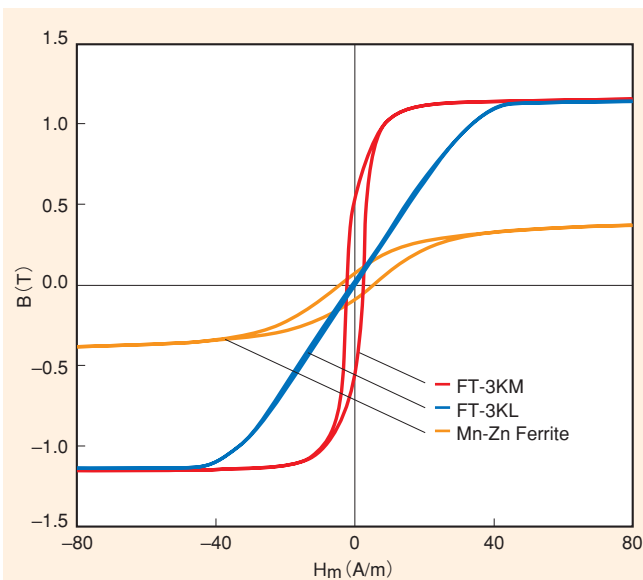
Figure 54. DC-BH Curves
