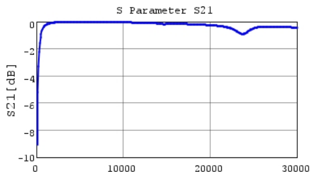
■ GJM0225C1C6R0WB01 S21 DCOV, 25degC
