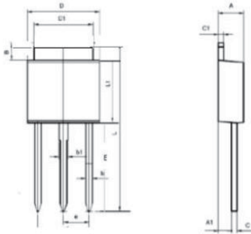
T0-251 (2)
