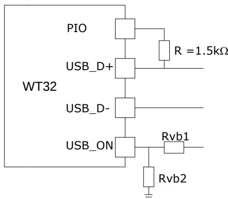
Figure 9: USB in self powered mode
