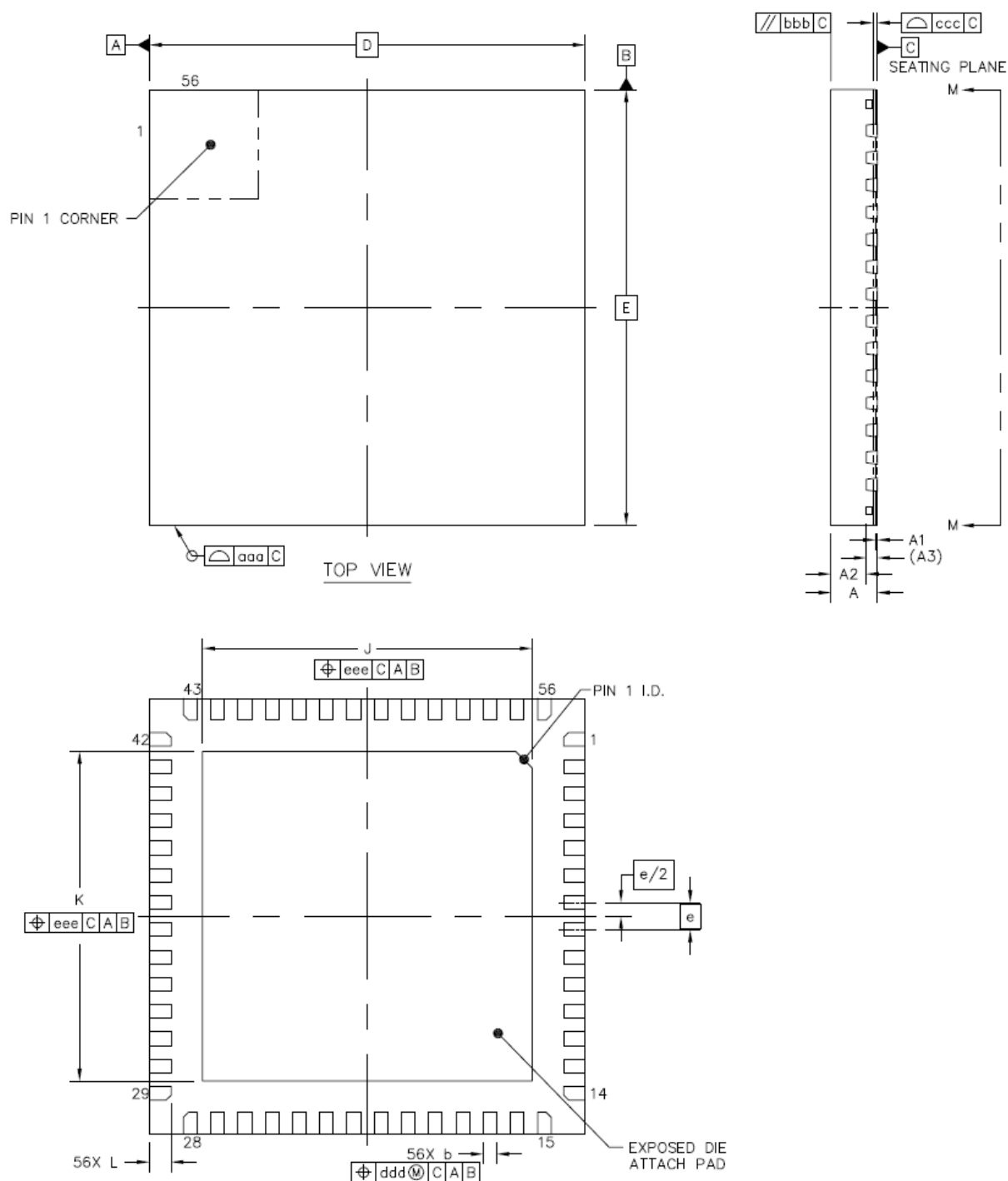
Figure 6.2. Package Drawing
