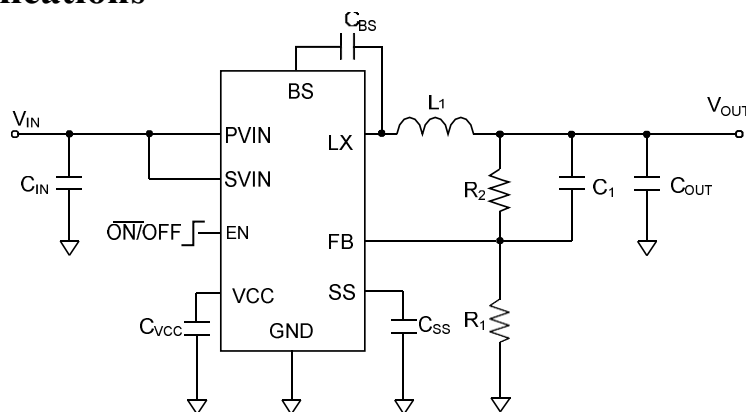
Figure 1. Schematic Diagram
