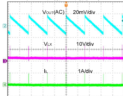
Output Ripple
