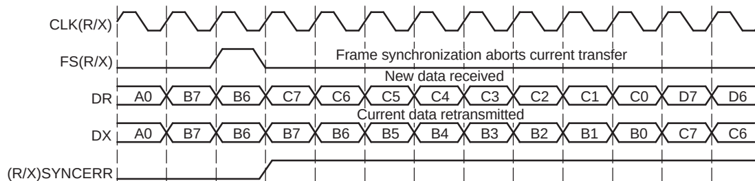
Figure 19-43. Unexpected Frame-Synchronization Pulse With (R/X)FIG = 0
