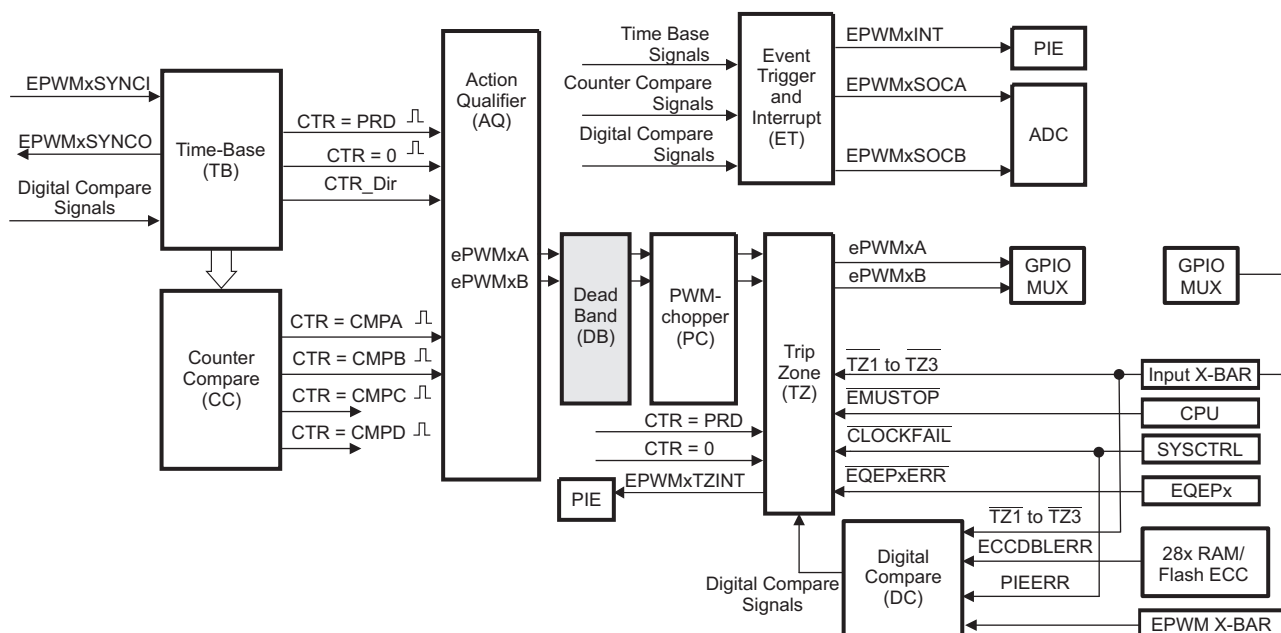
Figure 12-32. Dead_Band Submodule
