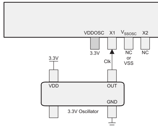
Figure 2-6. Single-ended 3.3V External Clock
