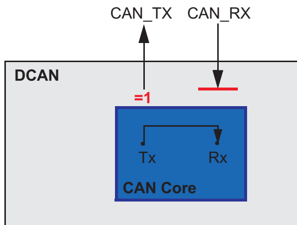
Figure 20-5. CAN Core in Loopback Combined with Silent Mode
