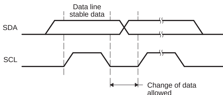
Figure 18-5. Bit Transfer on the I2C-Bus
