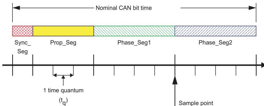
Figure 20-10. Bit Timing
