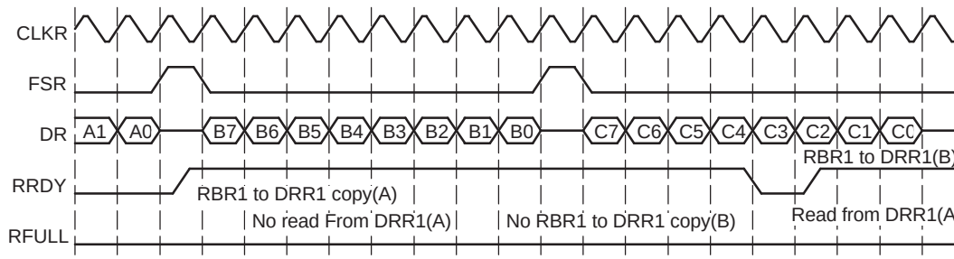
Figure 19-22. Overrun Prevented in the McBSP Receiver
