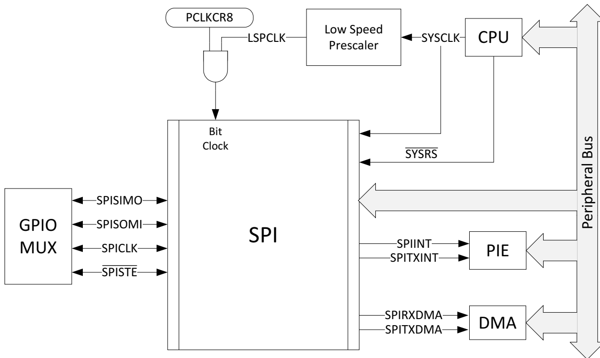
Figure 16-1. SPI CPU Interface
