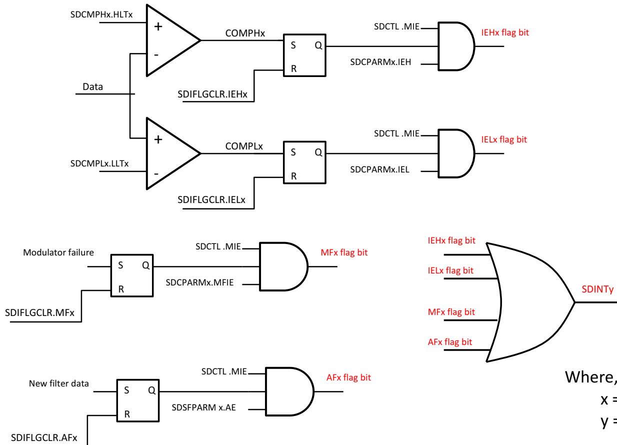
Figure 11-8. SDFM Interrupt Unit
