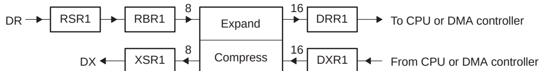
Figure 19-53. Companding Processes for Reception and for Transmission
