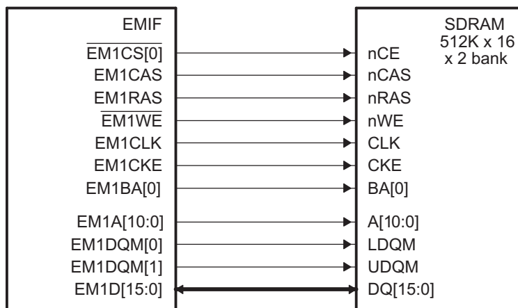
Figure 22-5. EMIF to 512K × 16 × 2 bank SDRAM Interface
