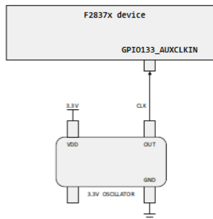
Figure 2-9. AUXCLKIN
