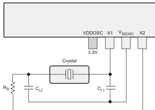
Figure 2-7. External Crystal
