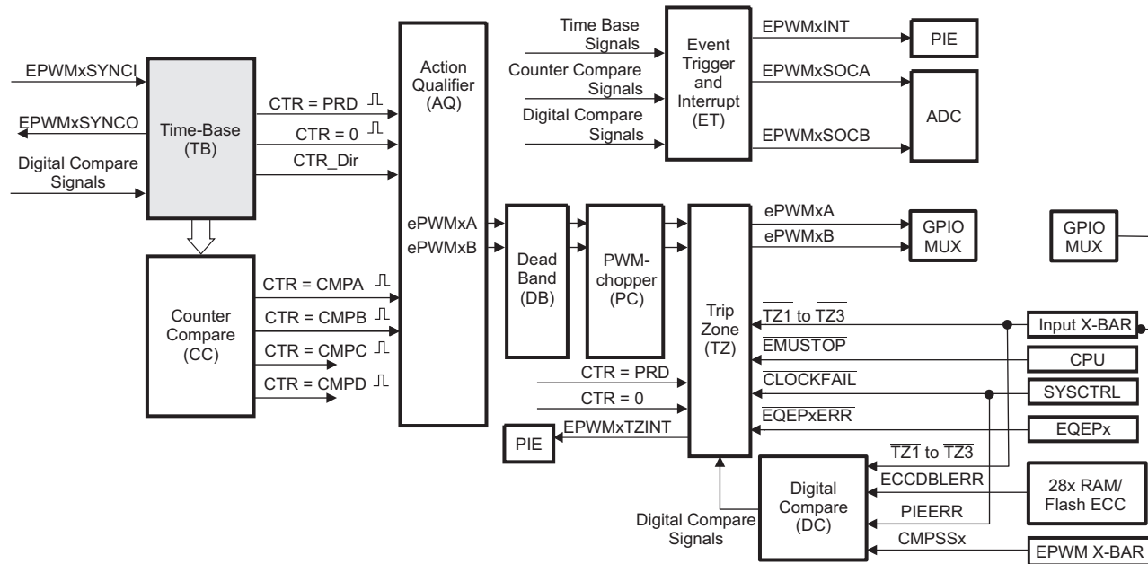
Figure 12-4. Time-Base Submodule
