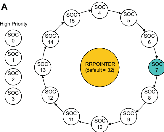
Figure 8-5. High Priority Example
