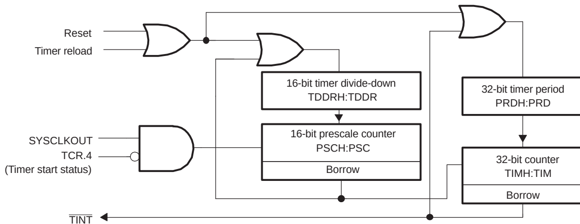
Figure 2-11. CPU-Timer Interrupts Signals and Output Signal
