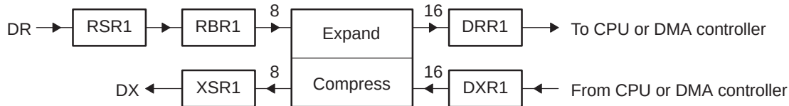
Figure 19-3. Companding Processes
