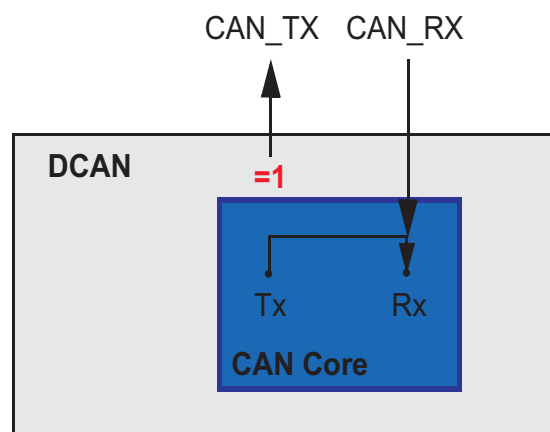
Figure 20-2. CAN Core in Silent Mode
