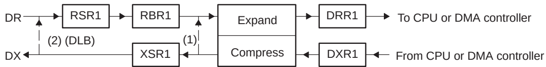
Figure 19-6. Two Methods by Which the McBSP Can Compand Internal Data
