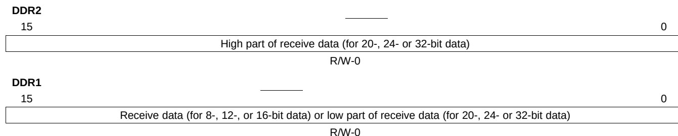
Figure 19-68. Data Receive Registers (DDR2 and DDR1)
