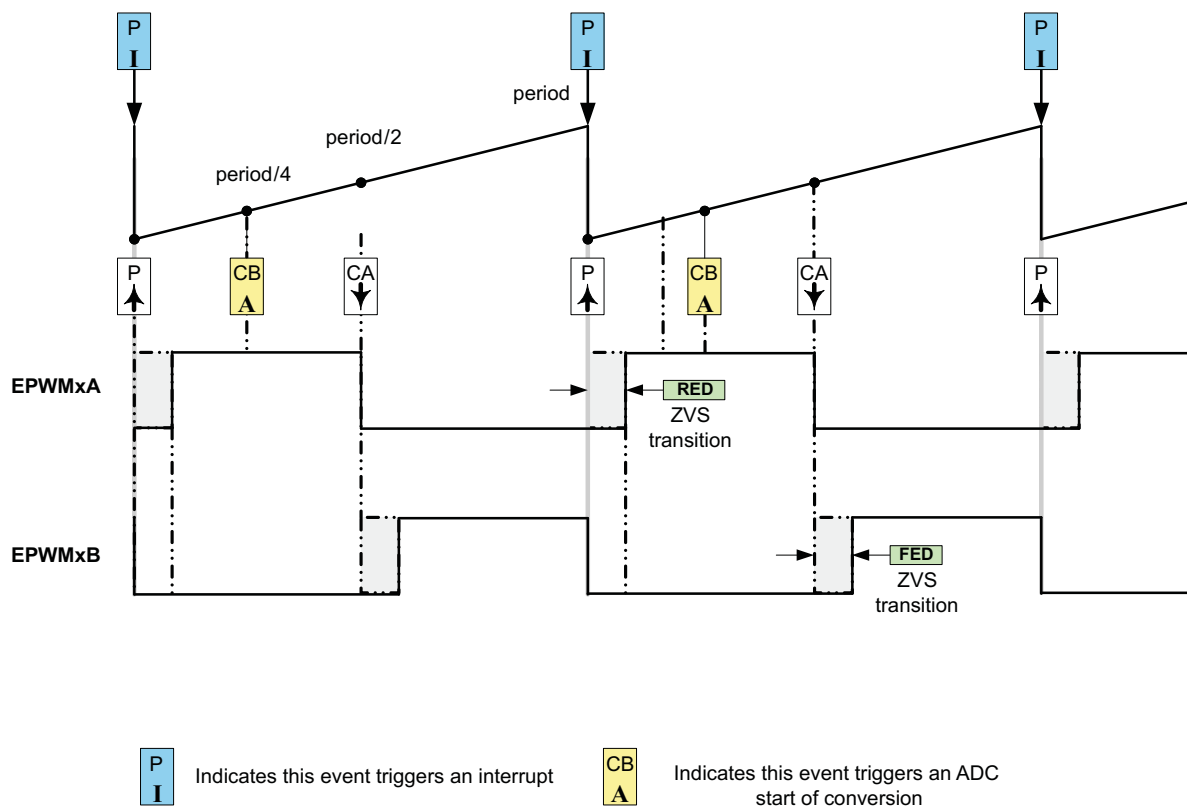
Figure 12-77. H-Bridge LLC Resonant Converter PWM Waveforms
