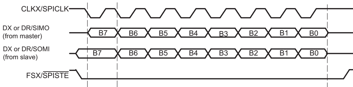
Figure 19-39. SPI Transfer With CLKSTP = 10b (No Clock Delay), CLKXP = 1, and CLKRP = 0
