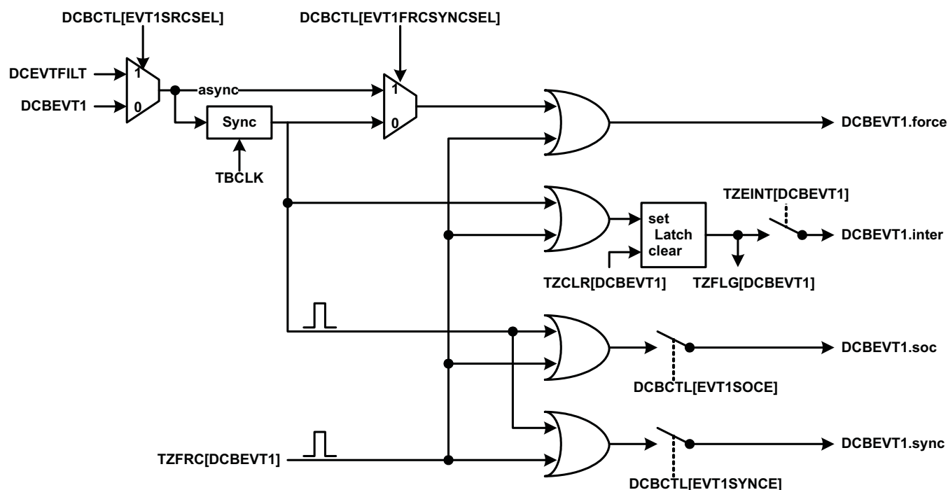
Figure 12-52. DCBEVT1 Event Triggering
