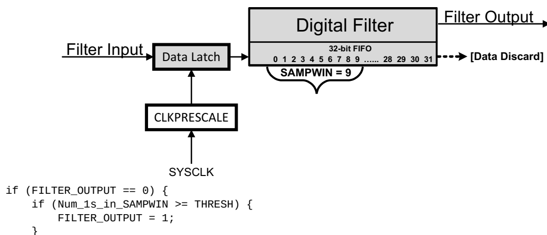
Figure 10-7. Digital Filter Behavior
