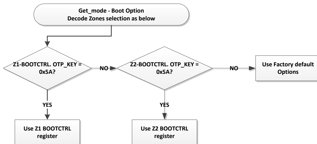
Figure 3-1. BOOTCTRL Selection
