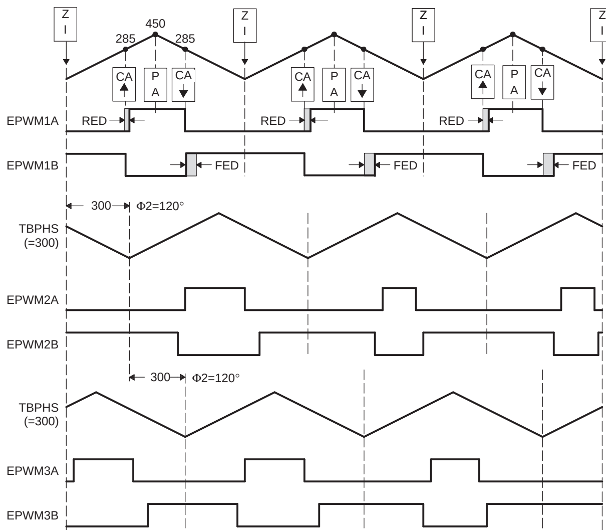
Figure 12-71. 3-Phase Interleaved DC/DC Converter Waveforms for Figure 12-70
