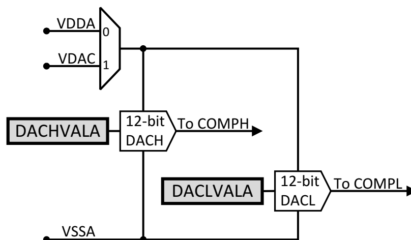
Figure 10-3. DAC Reference Select
