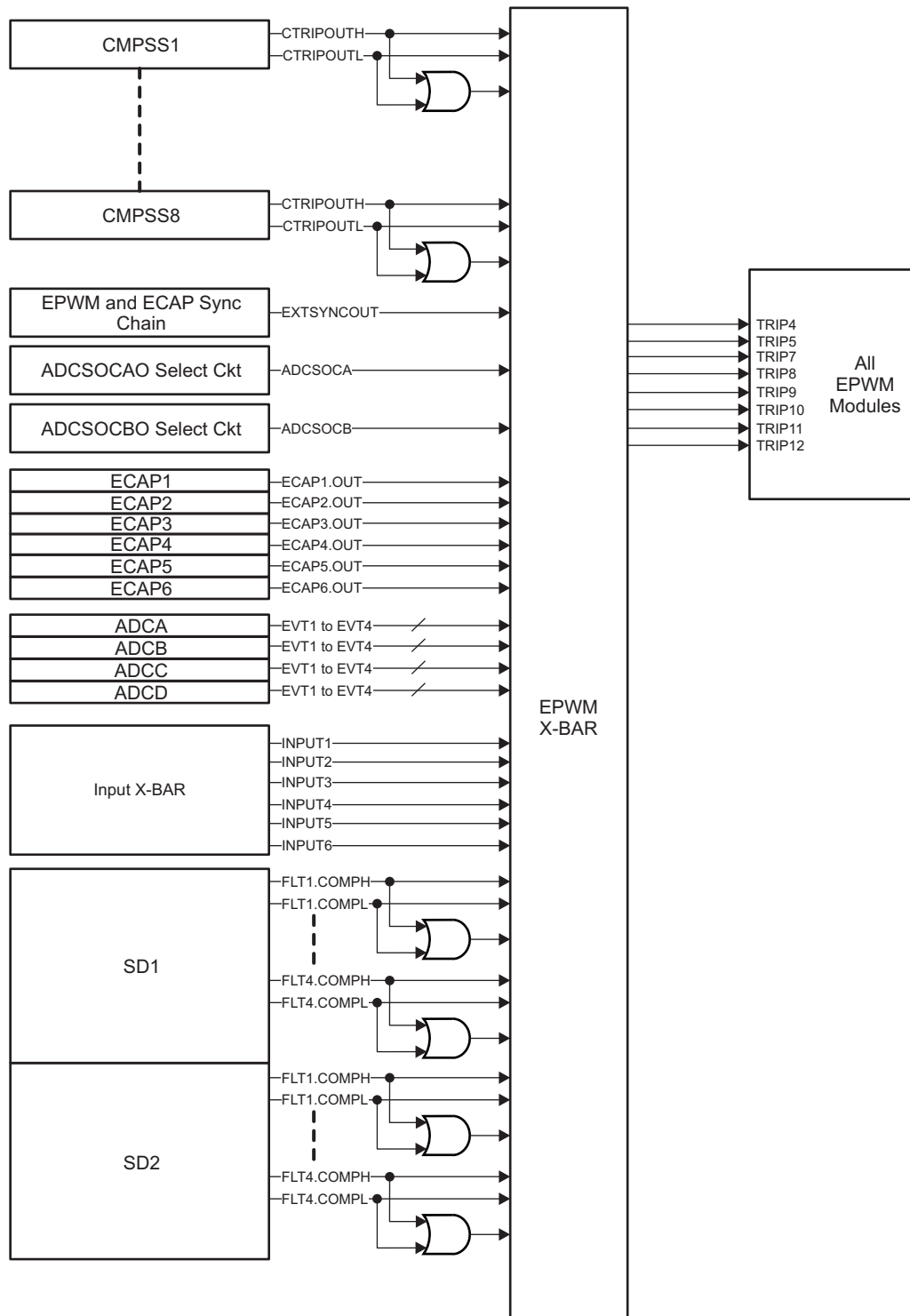
Figure 12-56. EPWM X-BAR
