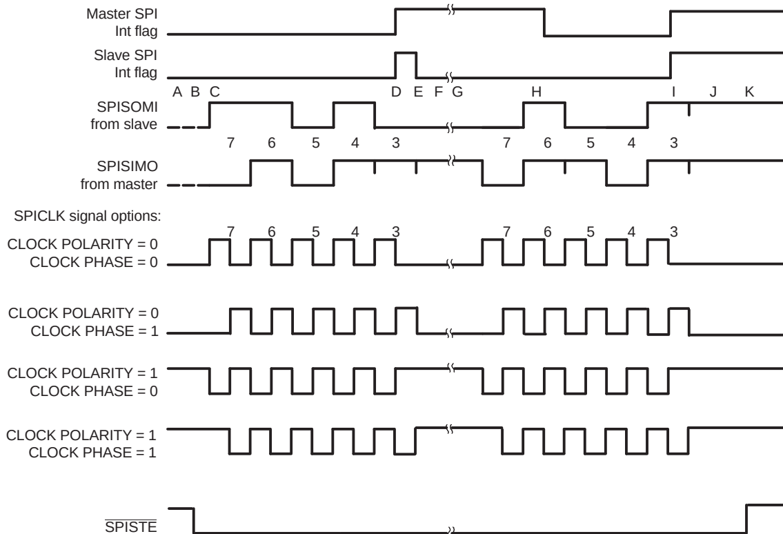
Figure 16-7. Five Bits per Character
