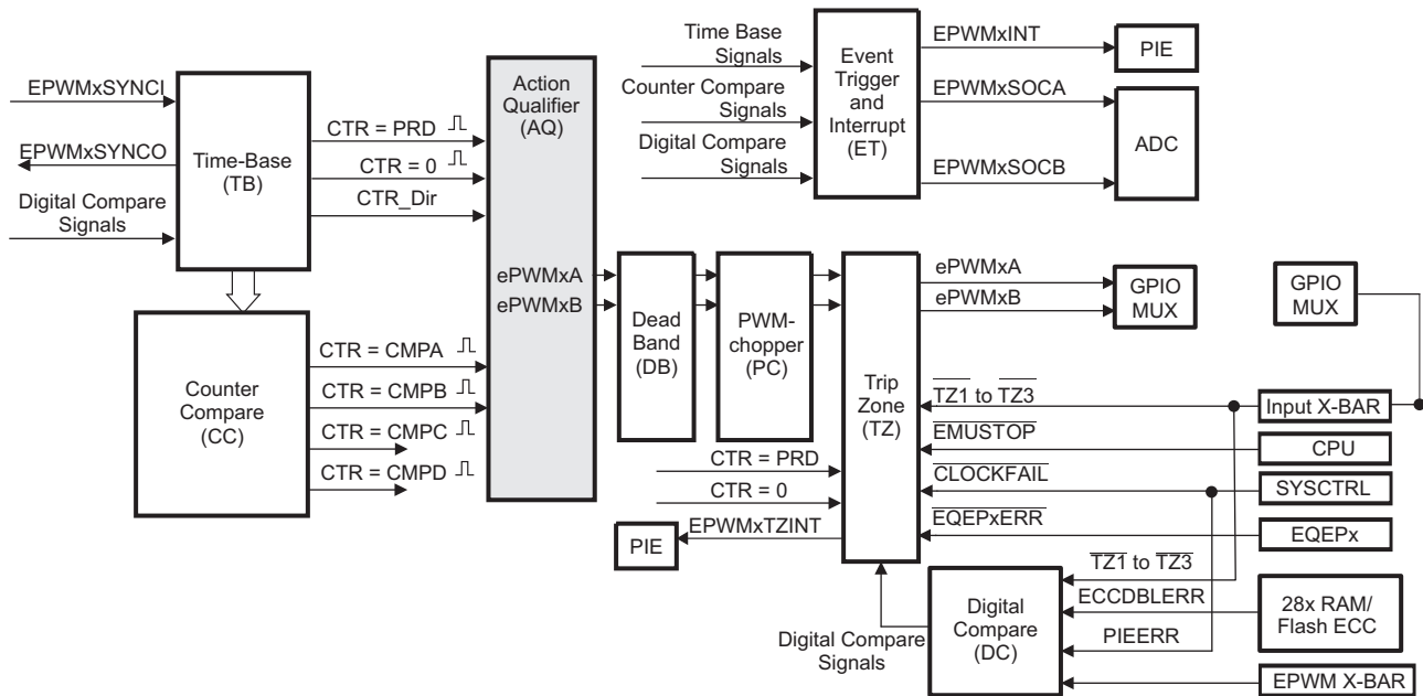
Figure 12-19. Action-Qualifier Submodule
