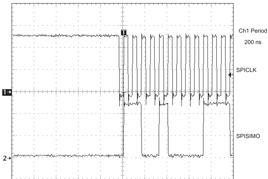
Figure 16-17. CLOCK POLARITY = 1, CLOCK PHASE = 1 (All data transitions are during the falling edge, but delayed by half clock cycle. Inactive level is high.)
