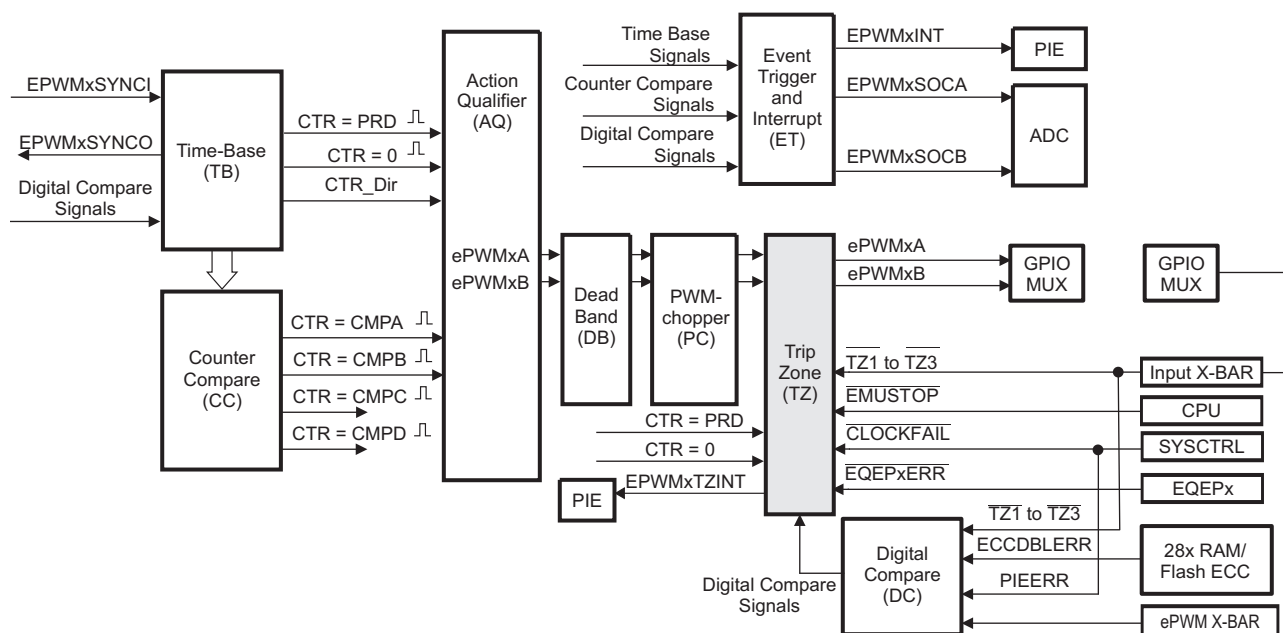
Figure 12-40. Trip-Zone Submodule
