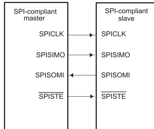
Figure 19-36. Typical SPI Interface
