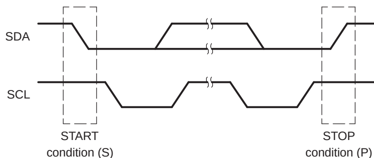
Figure 18-6. I2C Module START and STOP Conditions
