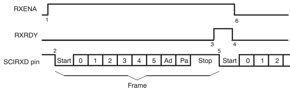
Figure 17-8. SCI RX Signals in Communication Modes
