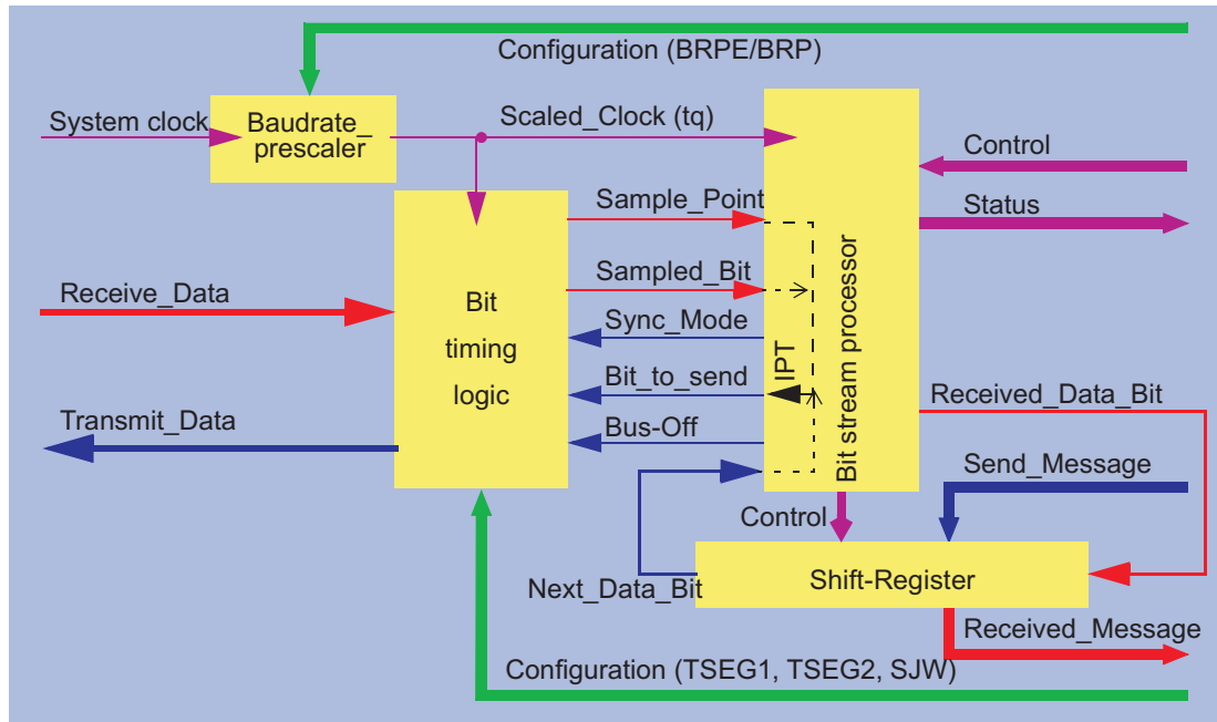
Figure 20-14. Structure of the CAN Core's CAN Protocol Controller
