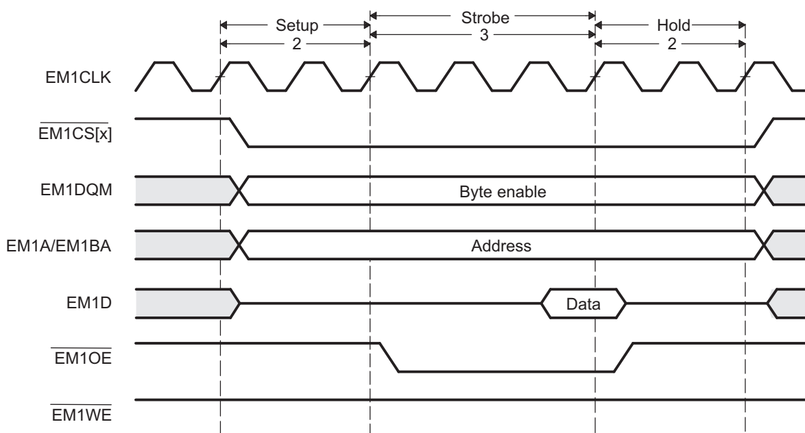
Figure 22-11. Timing Waveform of an Asynchronous Read Cycle in Normal Mode
