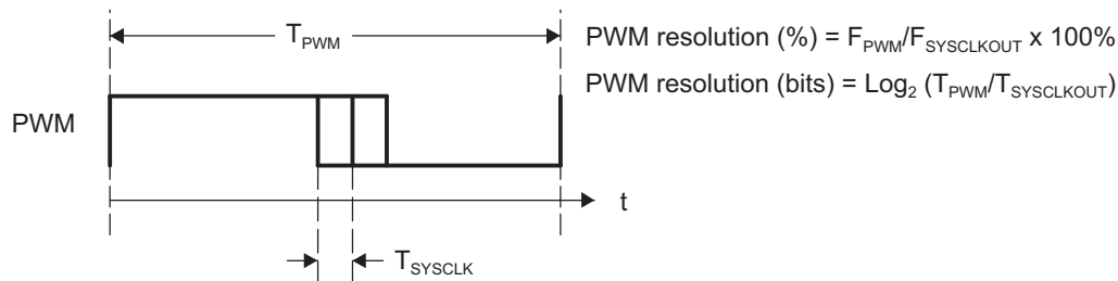
Figure 13-1. Resolution Calculations for Conventionally Generated PWM
