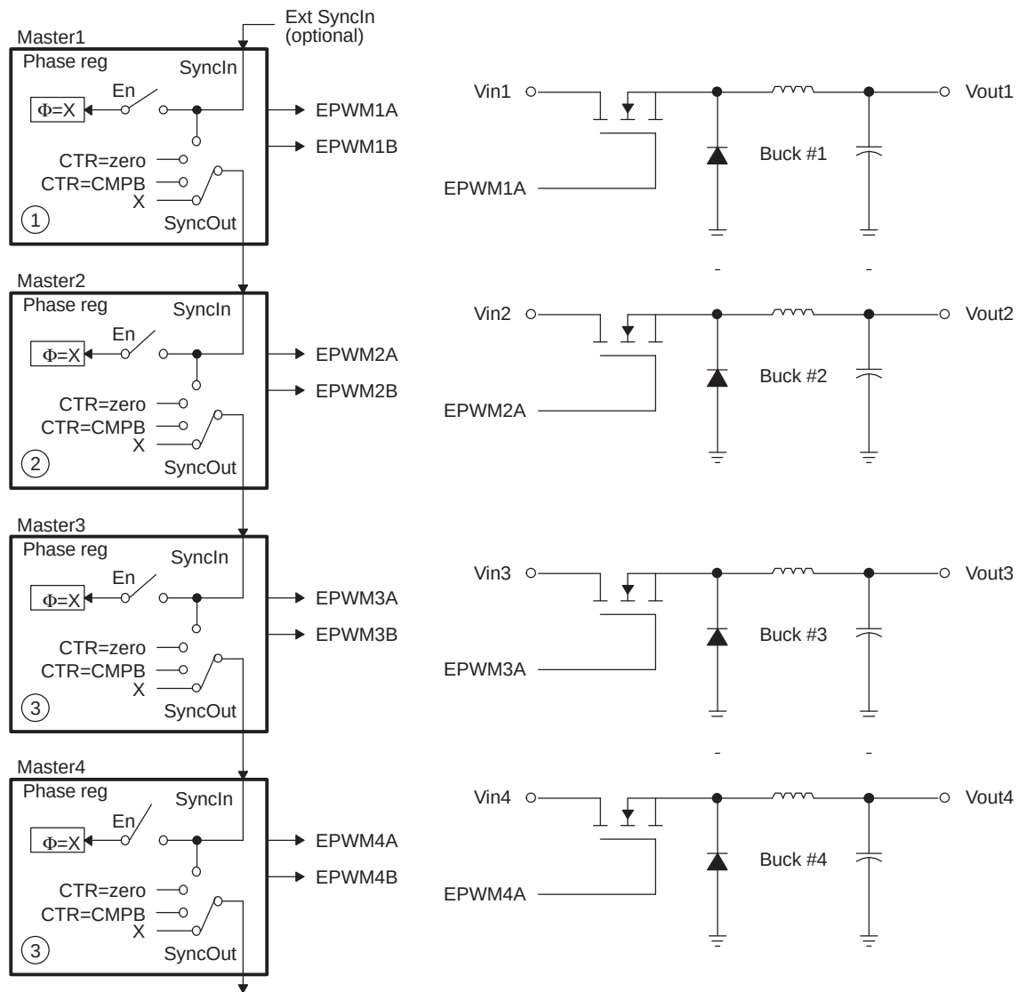
Figure 12-60. Control of Four Buck Stages. Here F_{PWM1} \neq F_{PWM2} \neq F_{PWM3} \neq F_{PWM4}
