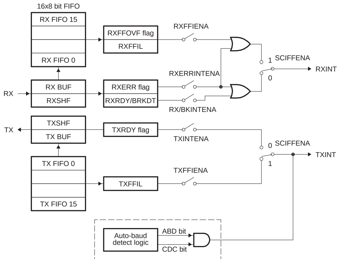
Figure 17-10. SCI FIFO Interrupt Flags and Enable Logic
