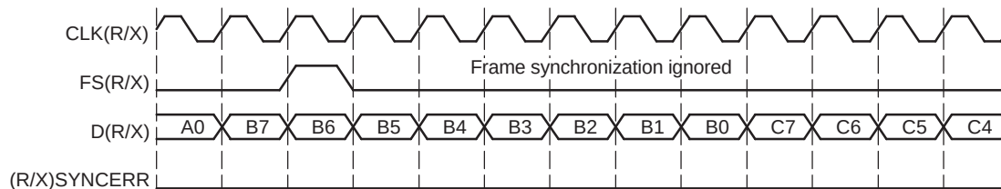
Figure 19-44. Unexpected Frame-Synchronization Pulse With (R/X)FIG = 1
