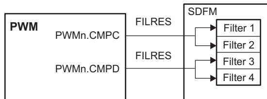
Figure 11-3. Typical PWM Interface to Sigma Delta Filter Module
