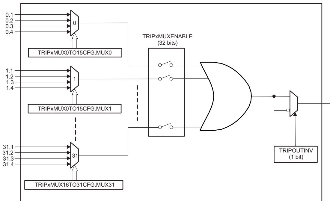
Figure 12-57. EPWM Architecture - Single Output
