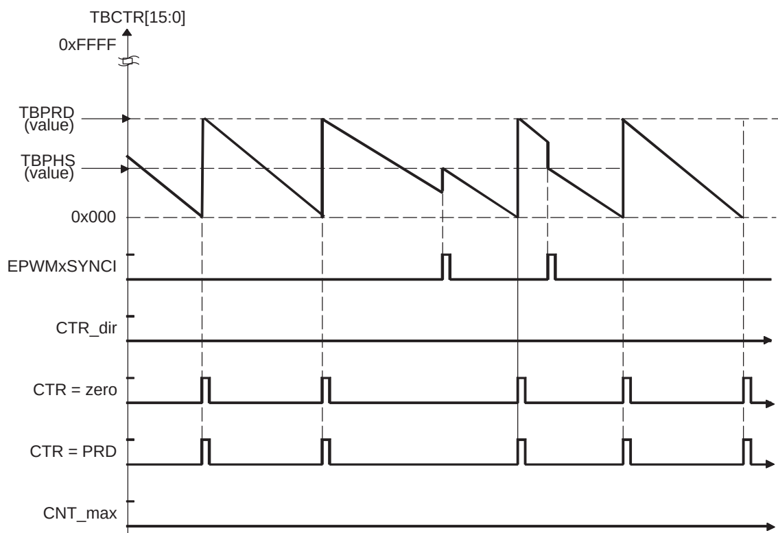
Figure 12-9. Time-Base Down-Count Mode Waveforms
