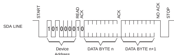
Figure 3-17. Sequential Read
