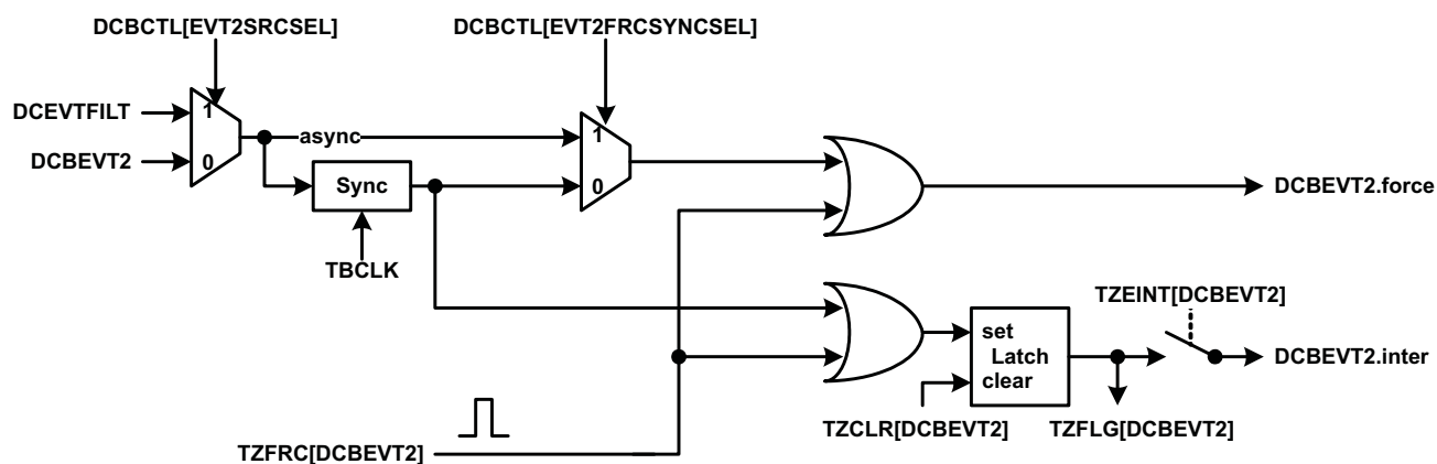
Figure 12-53. DCBEVT2 Event Triggering
