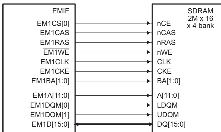
Figure 22-4. EMIF to 2M \times 16 \times 4 bank SDRAM Interface
