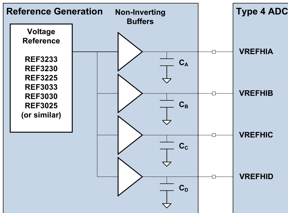
Figure 8-12. Shared Reference System
