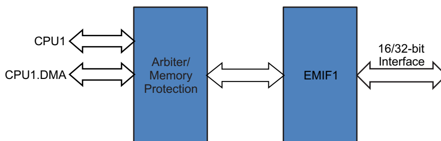
Figure 22-1. EMIF Module Overview
