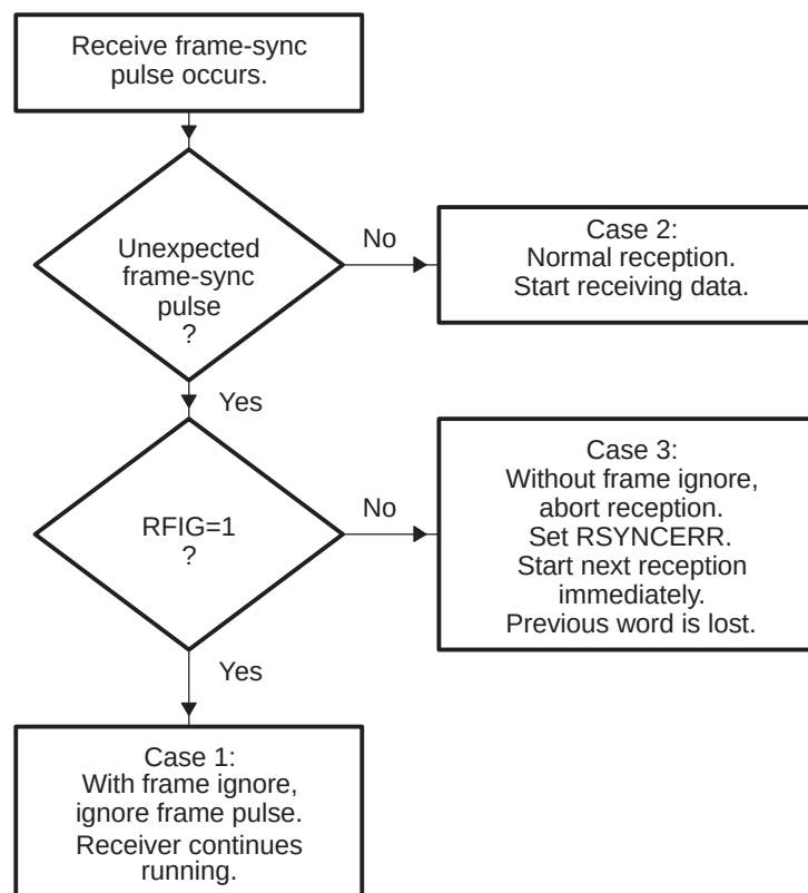
Figure 19-23. Possible Responses to Receive Frame-Synchronization Pulses
