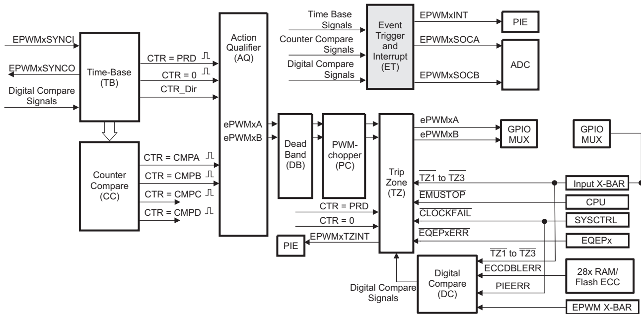
Figure 12-43. Event-Trigger Submodule
