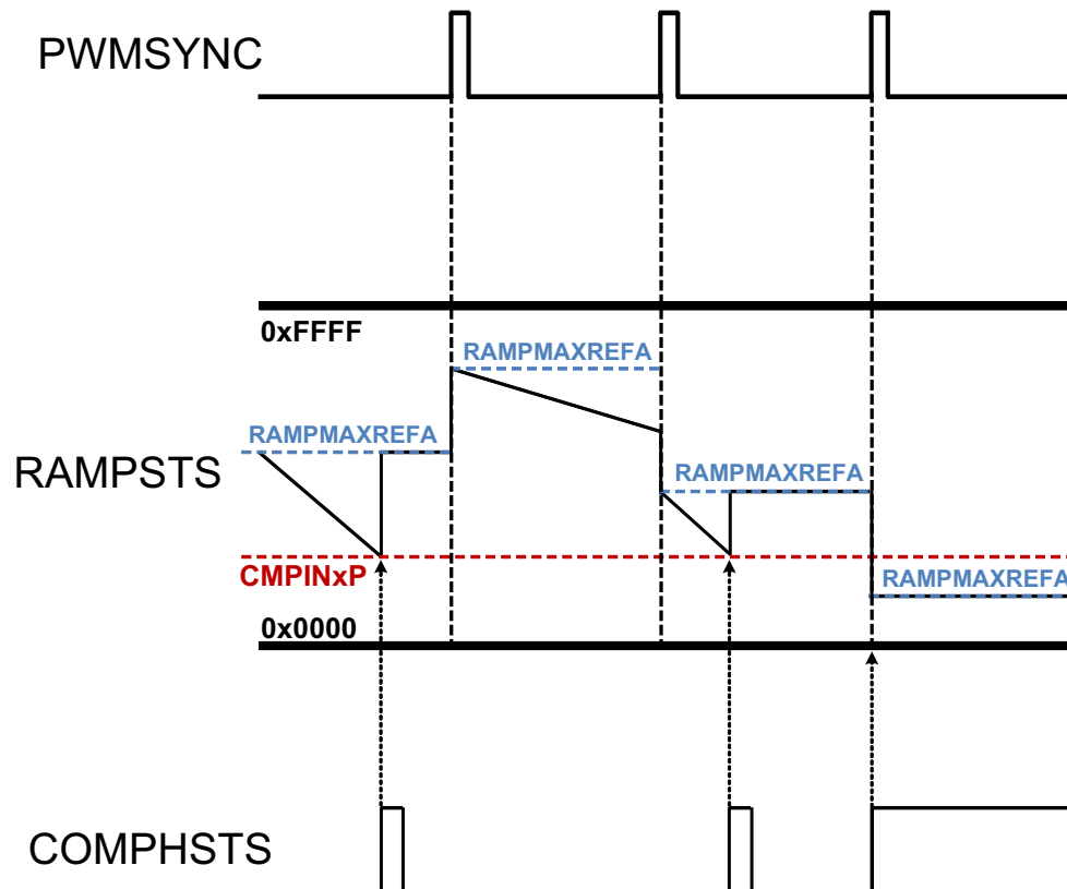
Figure 10-6. Ramp Generator Behavior
