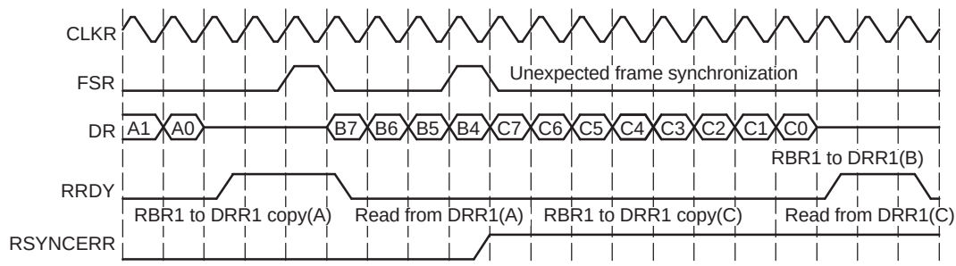
Figure 19-24. An Unexpected Frame-Synchronization Pulse During a McBSP Reception
