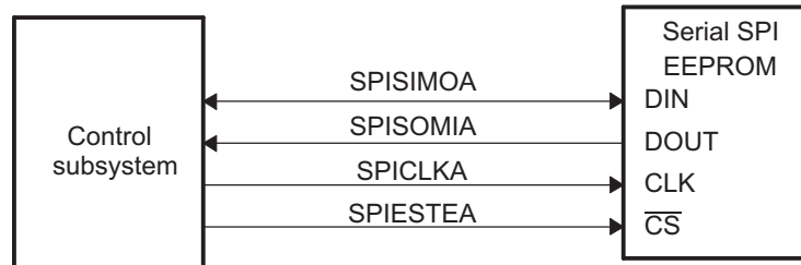
Figure 3-11. SPI Loader
