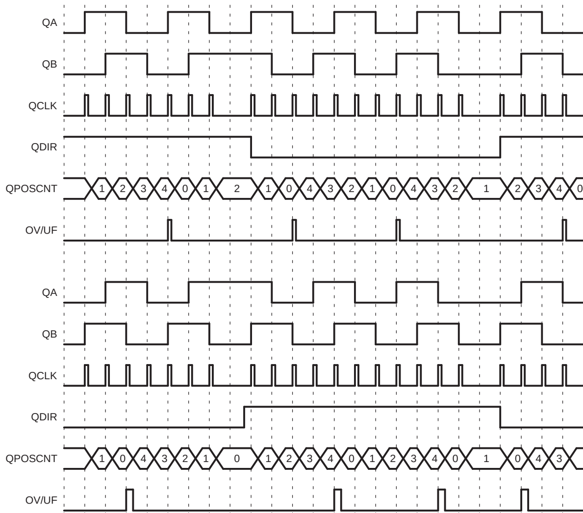
Figure 15-9. Position Counter Underflow/Overflow (QPOSMAX = 4)
