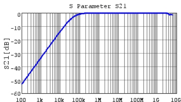
■ GCE21BR71H333KA01 S21 DC0V, 25degC
