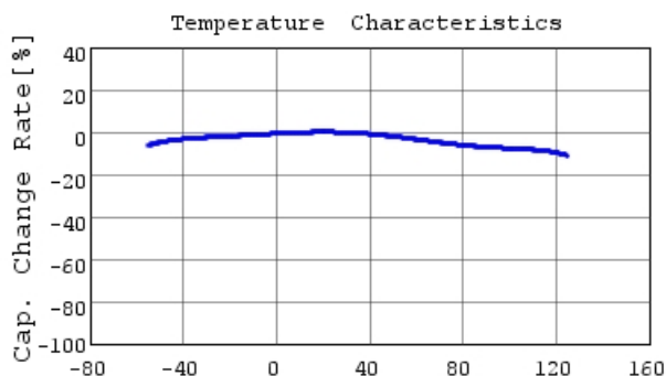
■ GCE21BR71H333KA01 C-Temp. capchange, DC0.0V,
