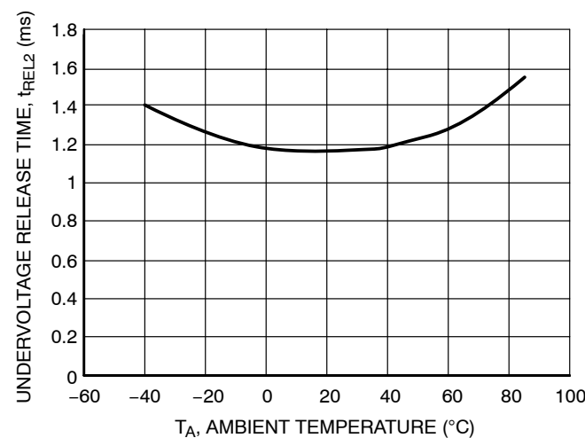
Figure 10. Undervoltage Release Time vs. Temperature
