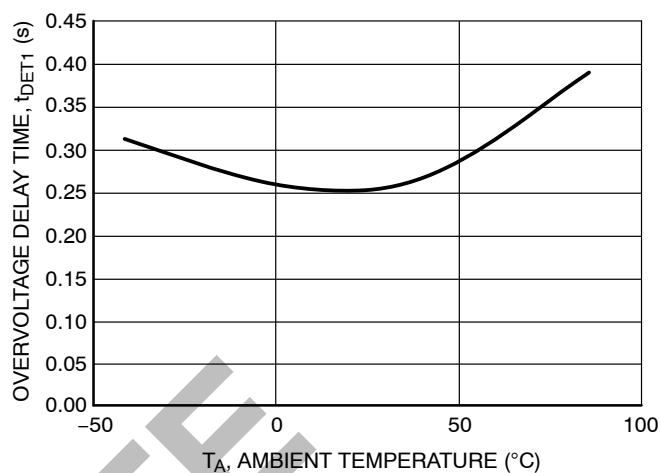
Figure 6. Overvoltage Delay Time vs. Temperature
