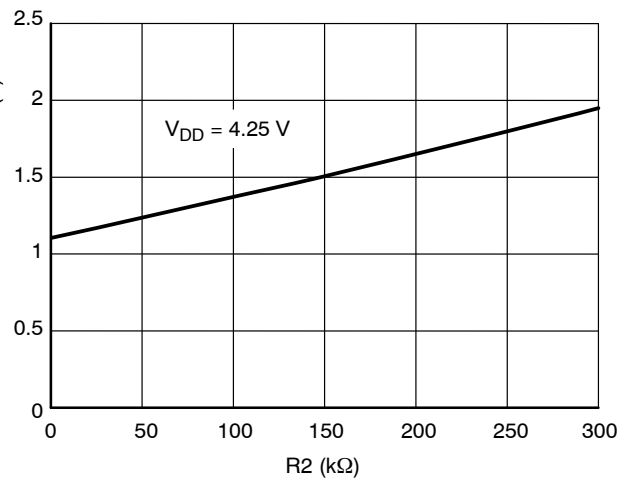
Figure 40. Charger Voltage to Release from Undervoltage vs. R2
