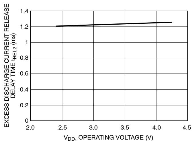
Figure 34. Excess Discharge Current Release Time vs. Operating Voltage
