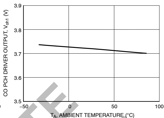
Figure 24. CO PCH Driver Output vs. Temperature
