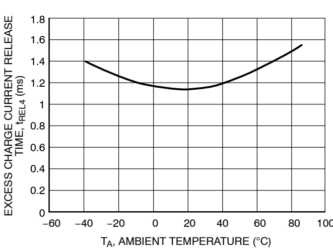
Figure 17. Excess Charge Current Release Time vs. Temperature
