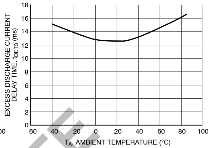
Figure 12. Excess Discharge Current Delay Time vs. Temperature
